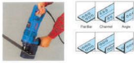
Model : HPC-18 Max. hole diameter 18mm (23/32") on 6mm (15/64") thickness
